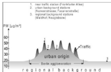
Figure 2: Horizontal profile for PM 10 concentration, Lenschow et al. (2001) – Atmospheric Environment 35, 29-33.
