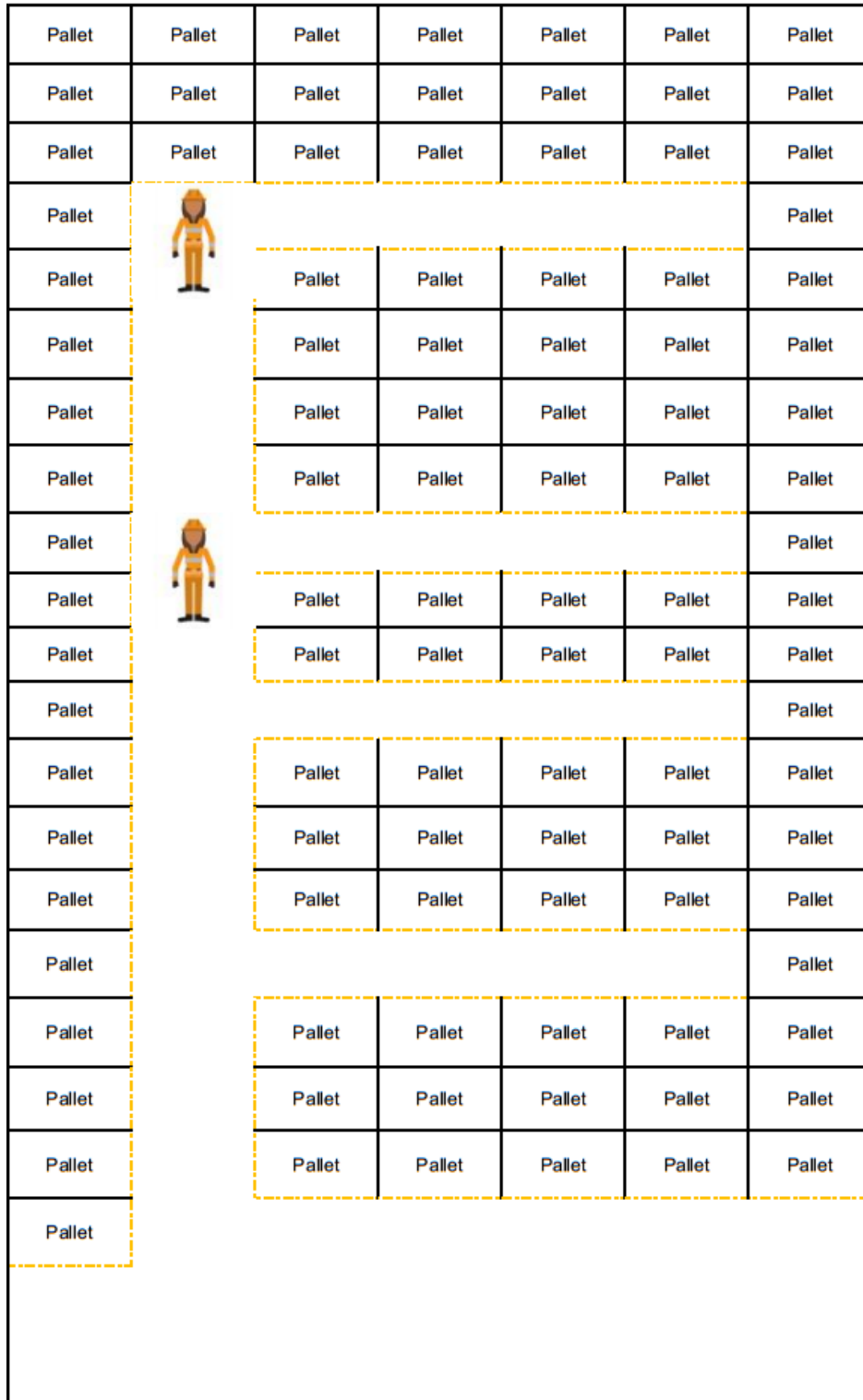
Fig 2.2: Internal Site Layout Plan of the facility, ), for the carrying out of the activities specified in condition 1.1.1. The extent of the site boundary is indicative and should not be used for interpretation purposes.
