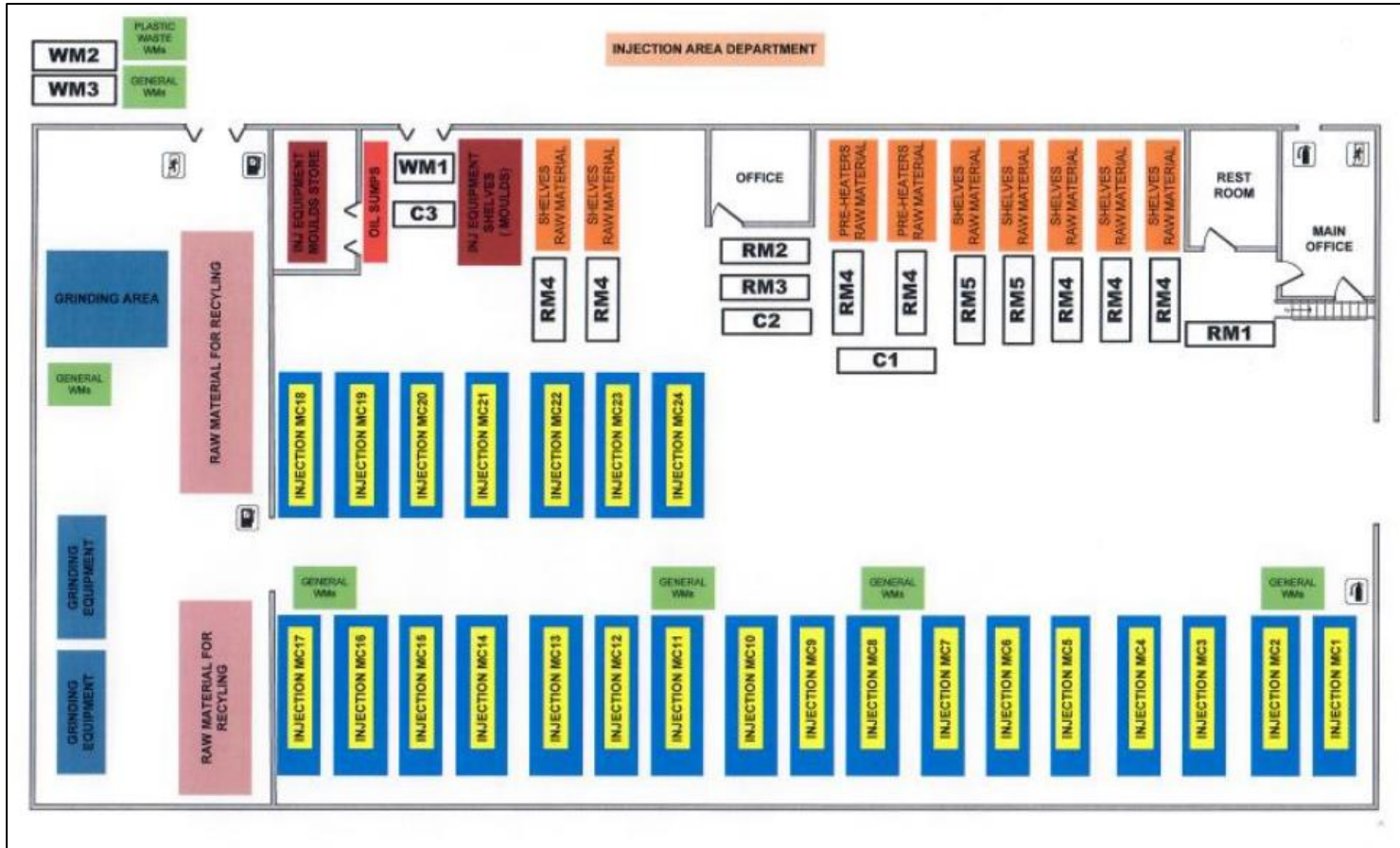
Fig. 2.3: Site layout plan for the carrying out of the activities specified in condition 1.1.1. The extent of the site boundary is indicative and shall not be used for interpretation purposes.
