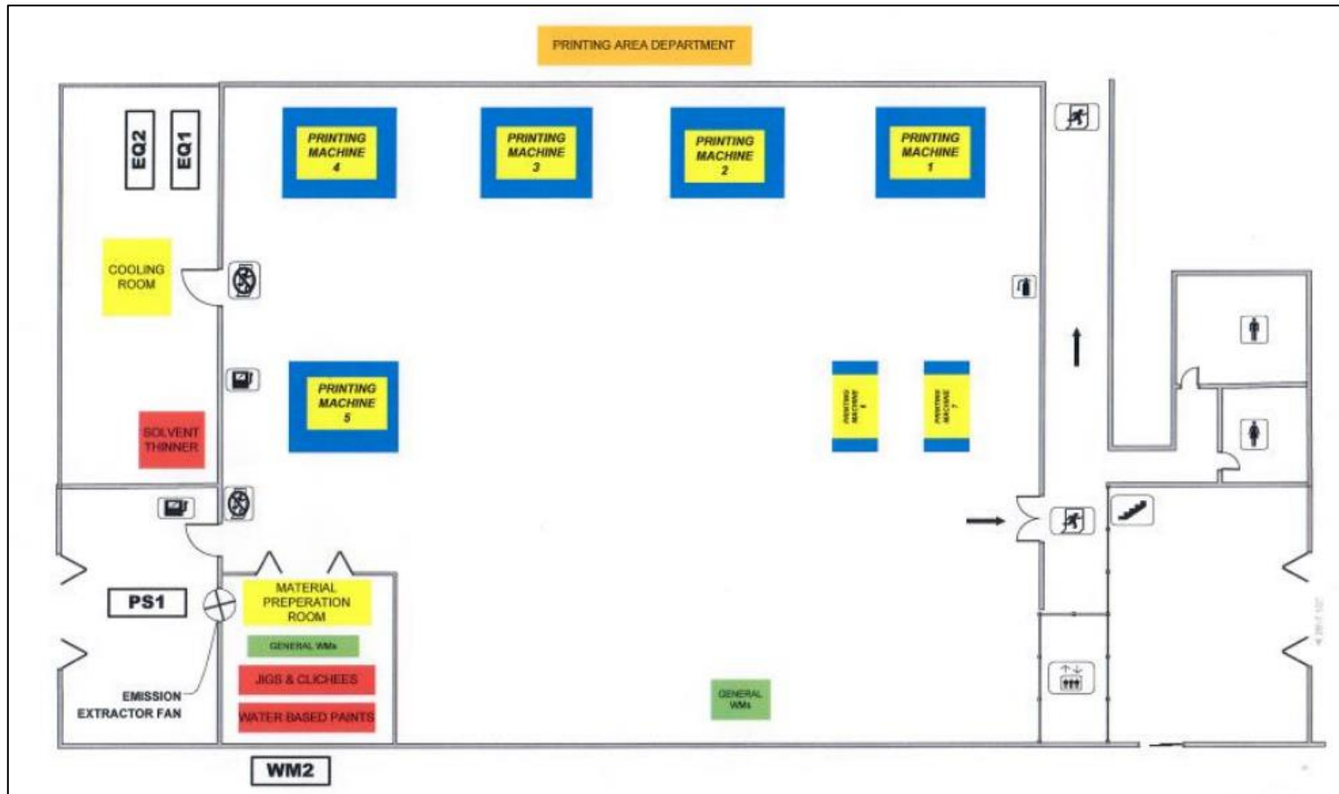
Fig. 2.2: Site layout plan for the carrying out of the activities specified in condition 1.1.1. The extent of the site boundary is indicative and shall not be used for interpretation purposes.
