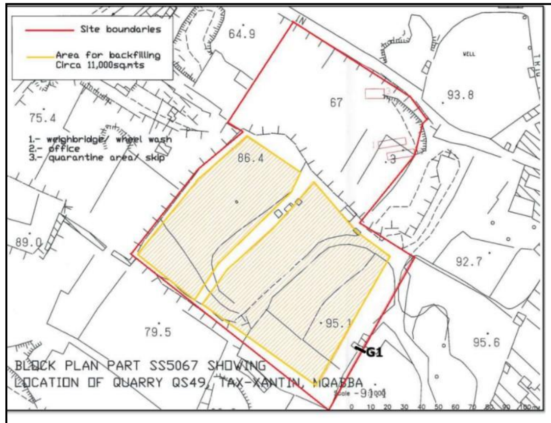
Fig. 3.1: Site of installation outlined in red, showing extent of area authorised for the carrying out of the activities specified in Condition 1.1.1. The extent of the site boundary is indicative and shall not be used for interpretation purposes.
