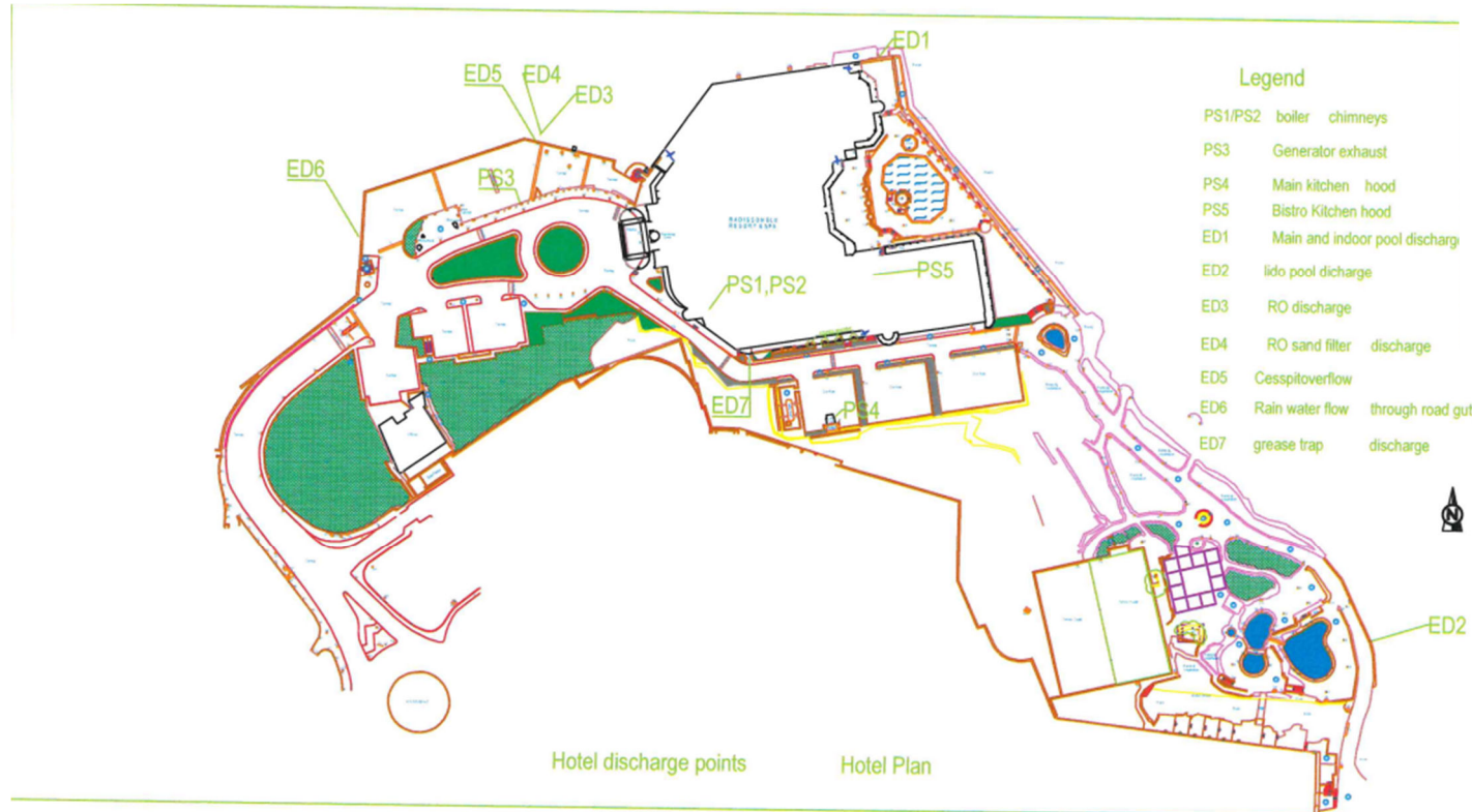
Fig. S1.4: Site layout of the permitted installation to undertake the activities specified in condition 1.1.1, showing emission points to the air and sea. The extent of the site boundary is indicative and shall not be used for interpretation purposes.
