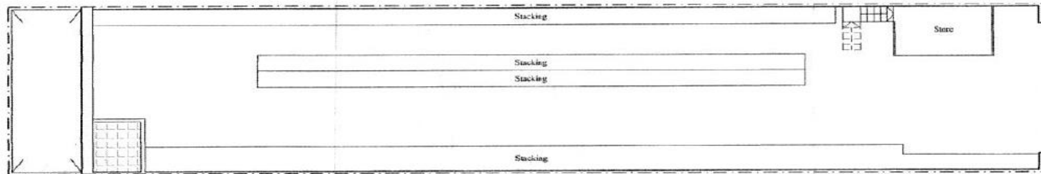
(P2 / D1) EXISTING INTERMEDIATE FLOOR PLAN Scale 1:100
