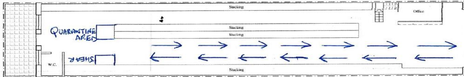
(P1 / D1) EXISTING GROUND FLOOR PLAN Scale 1:100
