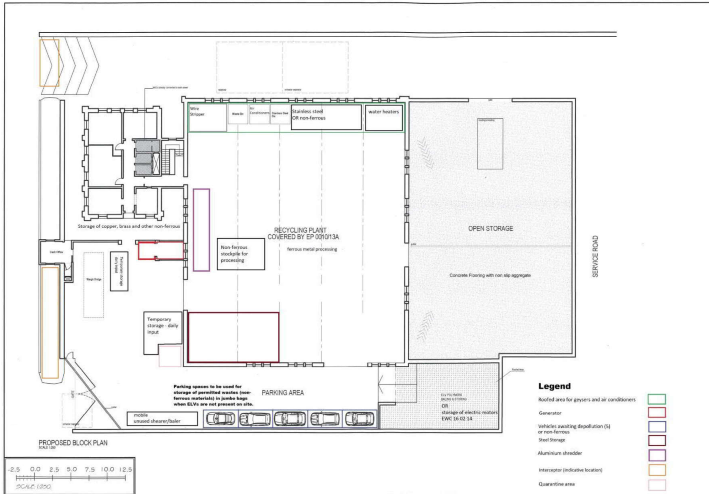
Figure 2.3: Site Layout showing the permitted upper level of the facility for the carrying out of the activities specified in condition 1.1.1. The extent of the site boundary is indicative and shall only be used for interpretation purposes.
