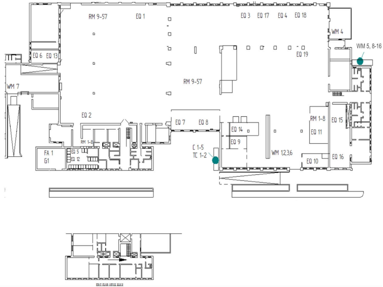
Figure S2.3: Site layout plan of installation for Phase 2 showing extent of area authorised for these operations and the location codes for Raw Materials (RM), Chemicals (C), Toxic Chemicals (TC), Equipment (EQ), Storage of Waste (WM), Generator (G) and Fuelling Area (FA). The extent of the site is indicative and shall not be used for interpretation purposes.
